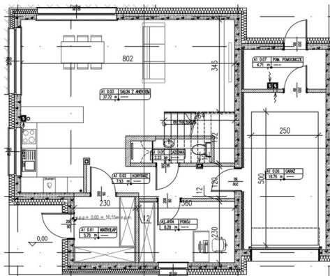
PARTER
